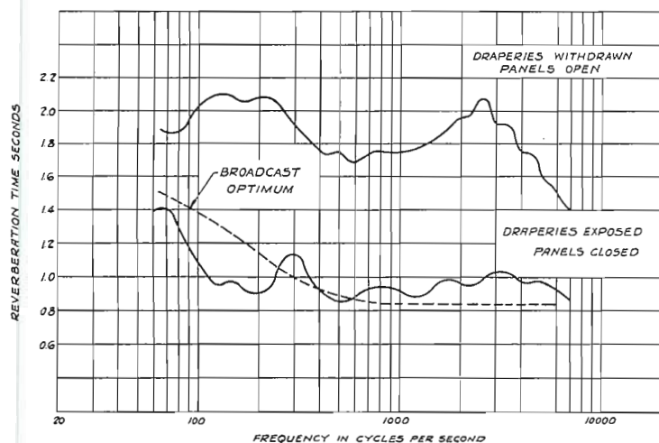
FIG. 4. Reverberation time-frequency characteristics.
