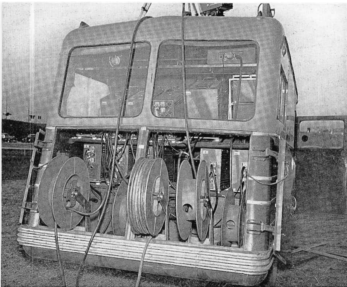
FIG. 7. (left) Rear view of unit showing how cable reels can be pulled out to facilitate unreeling. Inner end of cable extends through hole in reel to receptacle on camera control units on the operating table just above.
