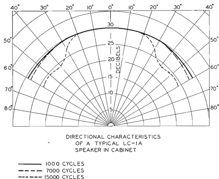
FIG. 5(a). Directional characteristics of the LC-1A Speaker at frequencies of 1,000, 7,000 and 15,000 cycles are shown in the diagram above. Note that the response is reasonably uniform over an angle of 120°.
