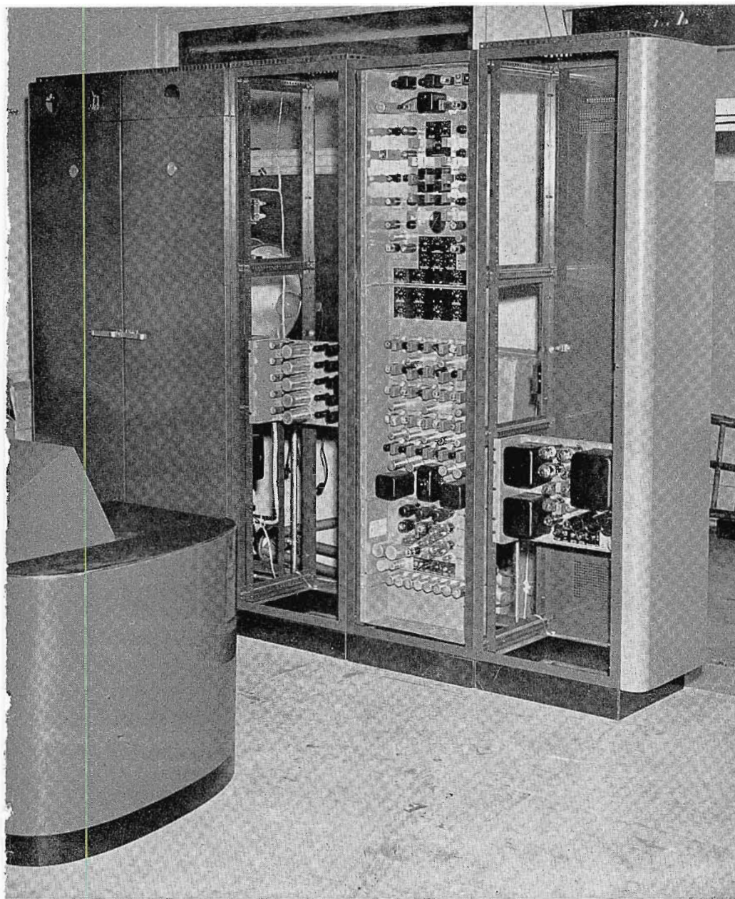
FIG. 3. (left) This photo, taken before installation of equipment was completed, shows the position of equipment racks which are located just behind the control console (a corner of which is visible). On these racks are mounted the main synchronizing generator, monoscope camera, distribution amplifier, and power supplies.
