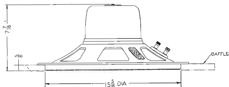
FIG. 8. Mounting dimensions for the LC-1A mechanism. Note the relatively thick mounting flange which is provided so that the thickness of the baffle board will not cause irregularities in the high-frequency response.
