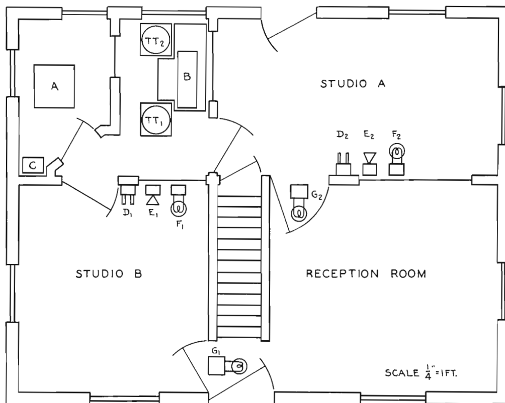
FIG. 7. Floor plan layout of the studios, control room, and transmitter room. Equipment items are as follows:
