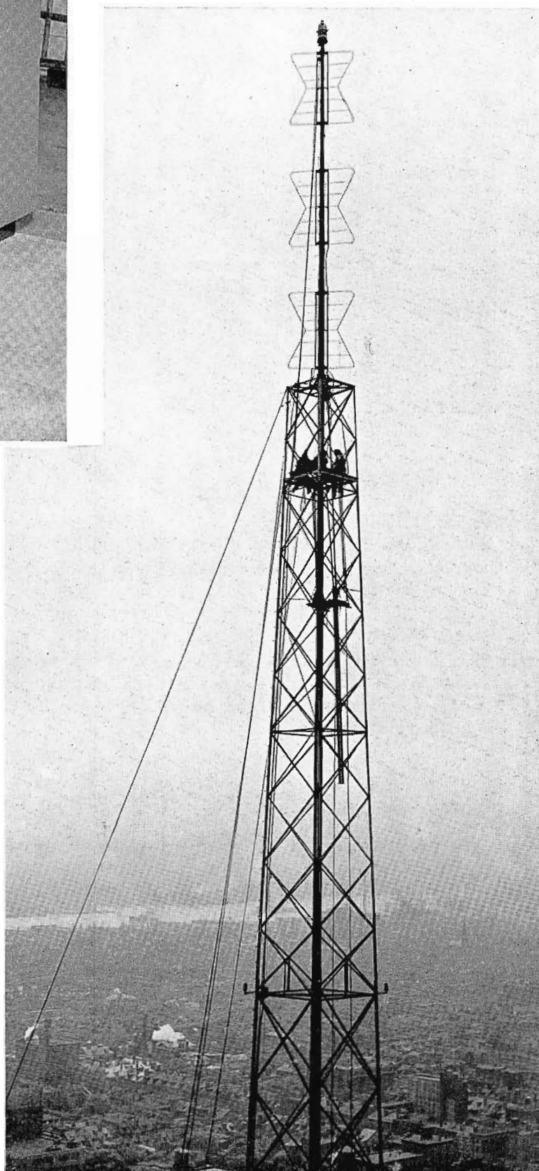
FIG. 4. (below) WFIL-TV's antenna, a three-bay RCA Super Turnstile, is mounted on a 200' tower atop the 18-story Widener Building opposite City Hall in the very center of Philadelphia. Antenna is 502' above the street.
