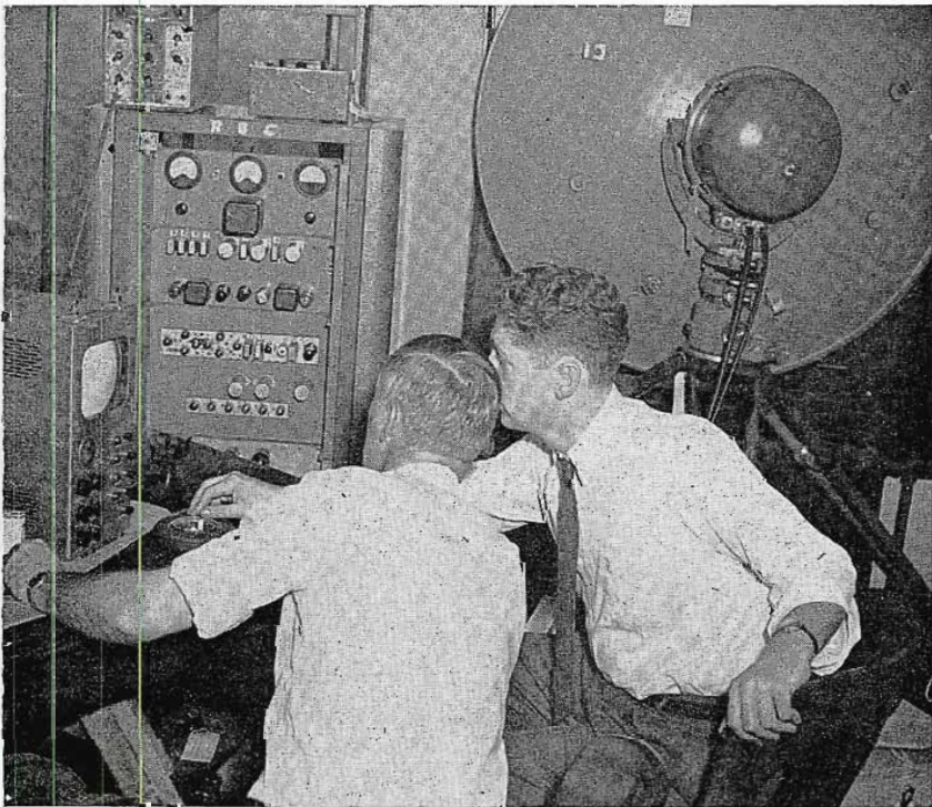
6. Video signal from the microwave transmitter was picked up by this RCA Microwave receiver located in the Lexington Building in downtown Baltimore. The output of this receiver fed the A. T. & T. coaxial cable to New York and Washington.
