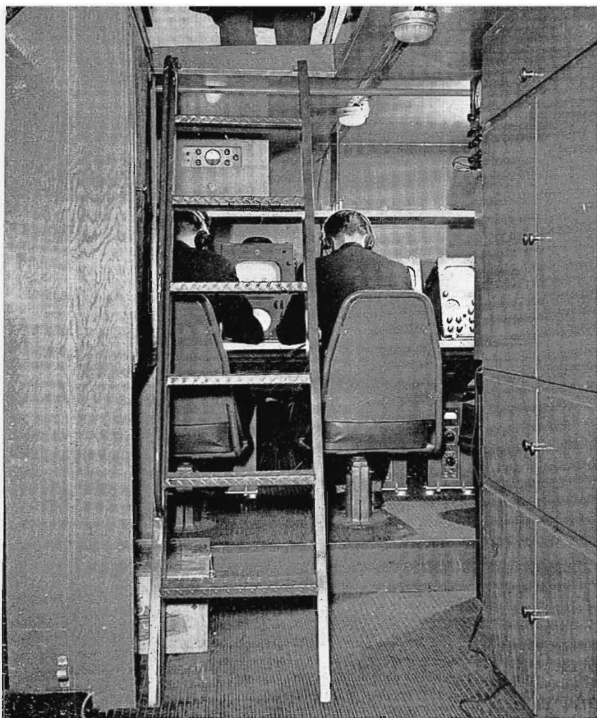
FIG. 3. (left) View inside the mobile unit, looking from the driver's seat toward the rear. Ladder, which provides easy access to the roof hatch, folds to ceiling when not in use. Cabinets at right provide carrying space for cameras, relay equipment, etc.
