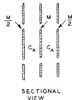
FIG. 3. Equivalent schematic and sectional view of acoustical filter.
