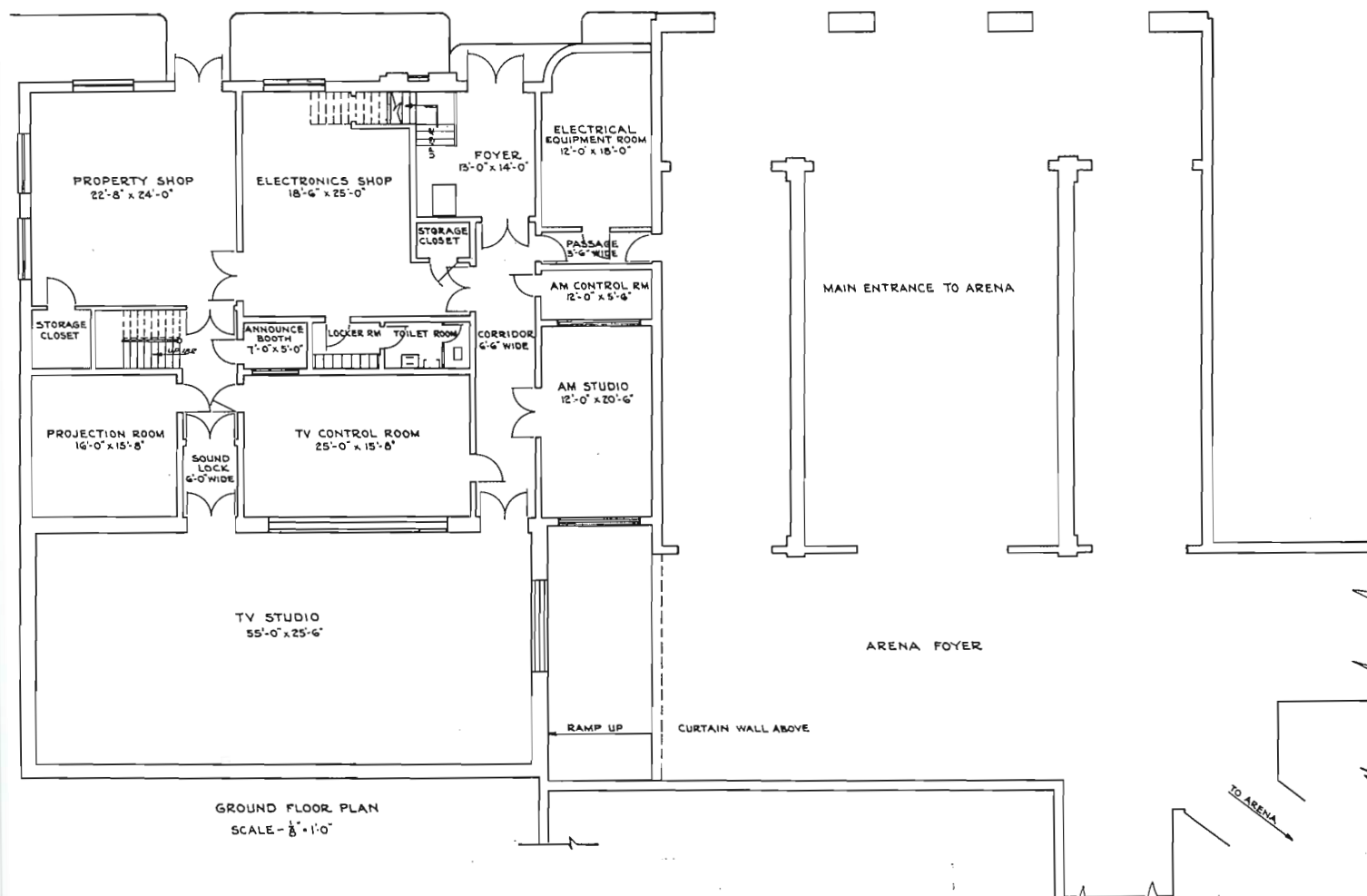
FIG. 6. (above) This is the ground floor layout of the new WFIL-TV Studio Building. Note window in the TV Studio through which visitors to the Arena will be able to watch television operations.
