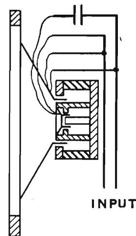
FIG. 3. Diagram showing relative mounting of the two cones in the LC-1A and the manner in which connections are made to the two-field coils.
