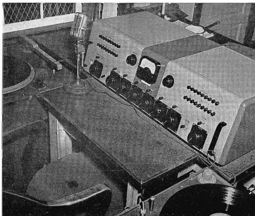
FIG. 8. Turntables are located in the control room as shown here, since there was no room for a separate announce booth. Microphone shown can be used for either talkback, or announcing.
