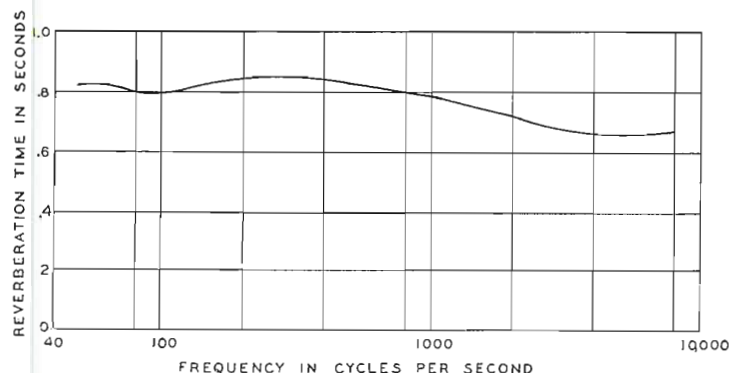
FIG. 2. Reverberation time-frequency characteristic of the test room.
