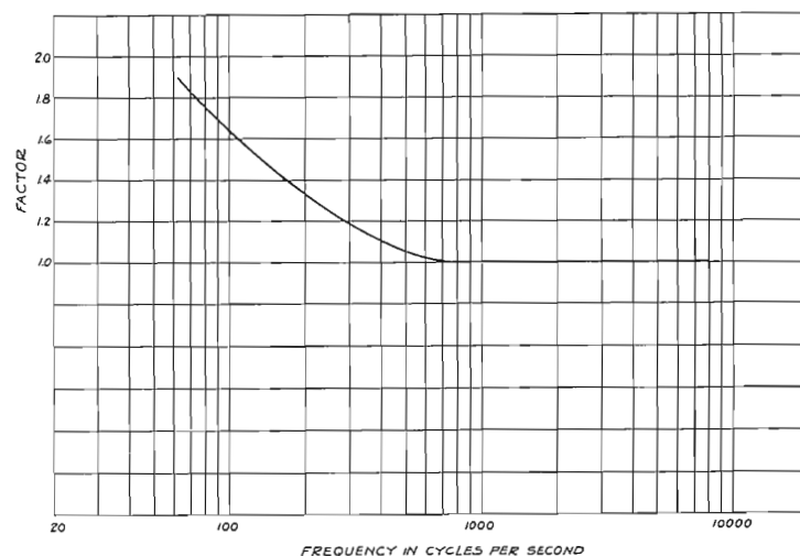
FIG. 5. Reverberation time-frequency ratio.
