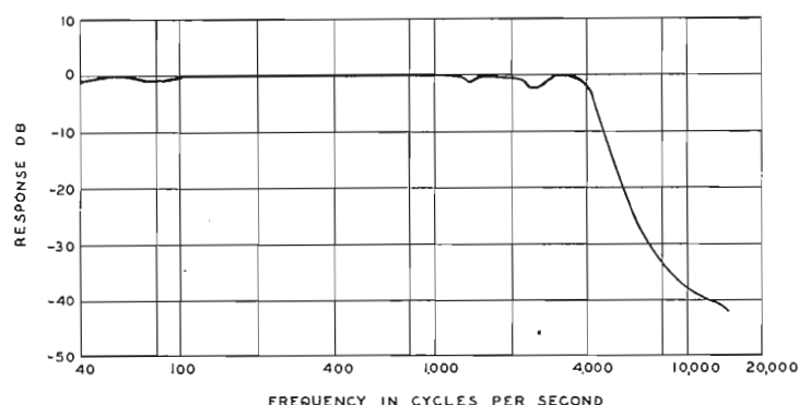
FIG. 6. The response-frequency characteristic of the acoustical filter.
