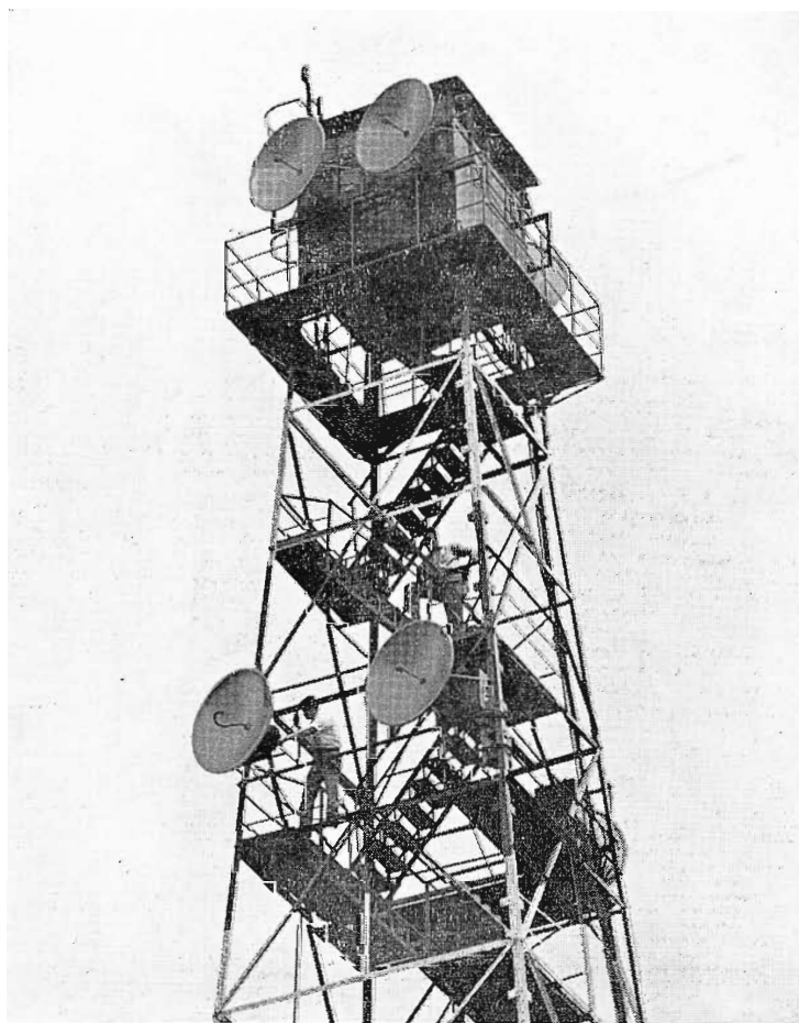
FIG. 2. Transmitter antenna (the parabola at lower left) mounted on Western Union Relay System tower at Bordentown, N. J., about 27 airline miles from the receiving antenna.
